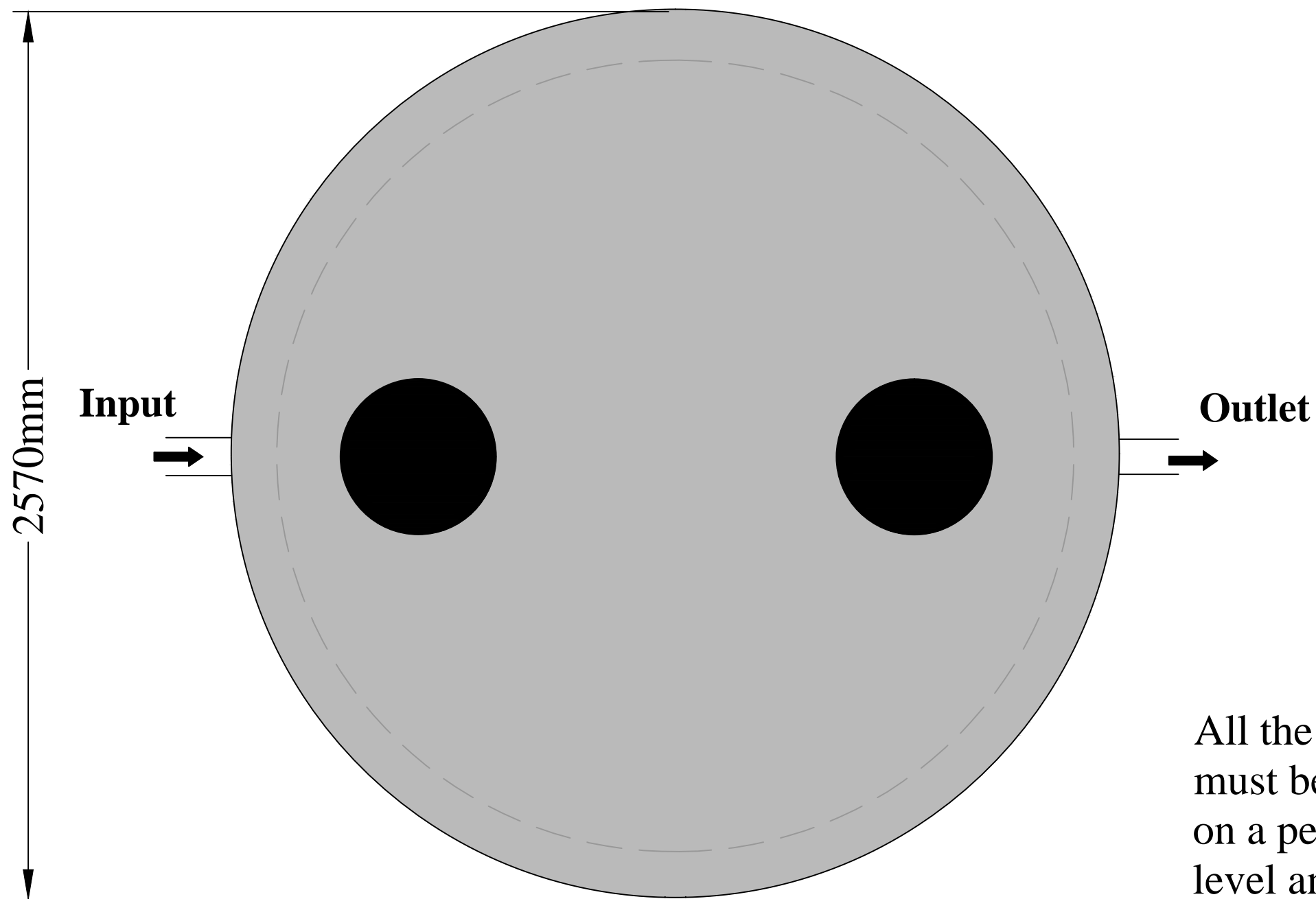
Tank Top Plan
