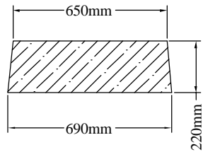
Riser Vertical Section
