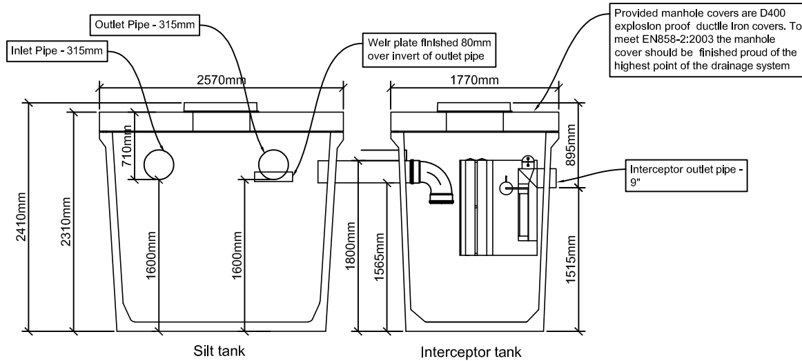
SECTION - Through A-A
